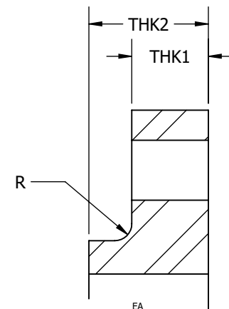
DETAIL B
