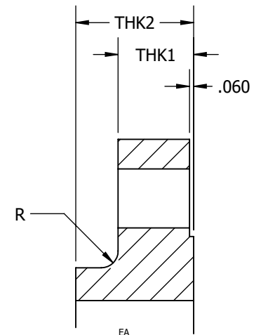
DETAIL B
